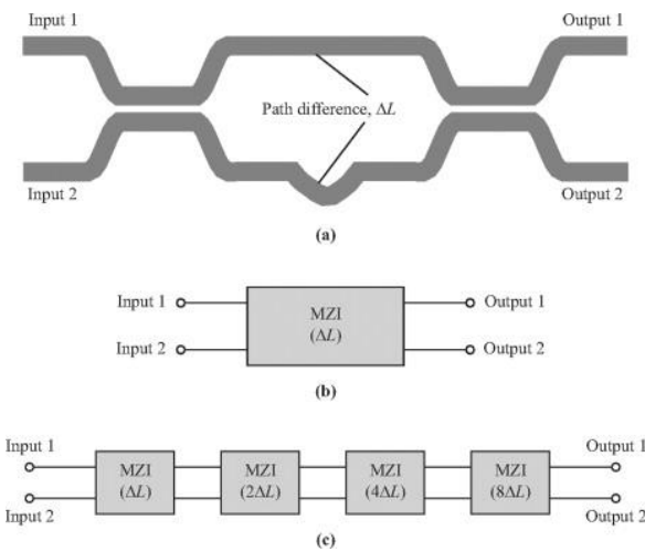
Figure 10 - (a) An MZI constructed by interconnecting two 3 dB directional couplers. (b) A block diagram representation of the MZI in (a). \Delta L denotes the path difference between the two arms. (c) A block diagram of a four-stage Mach-Zehnder interferometer, which
