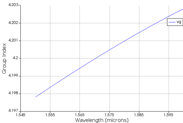
Figure 5 - Wave guide group index vs. wavelength
