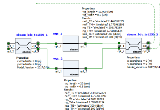
Figure 18 - Details of the parameters obtained in the simulation
