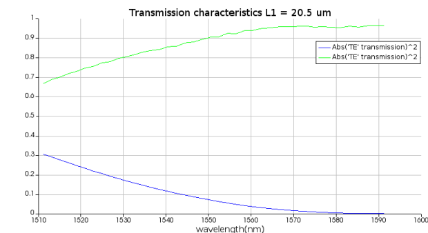
Figure 15 - Transmission characteristics L = 20.5 um
