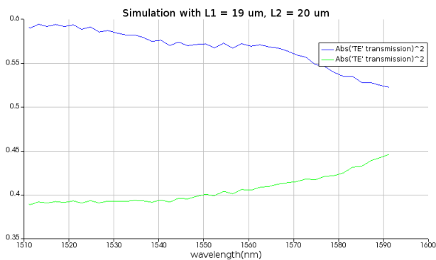
Figure 13 - Transmission characteristics L = 19 um
