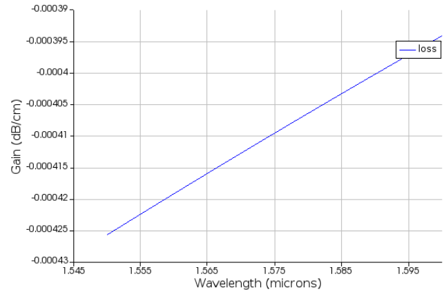
Figure 8 - Waveguide Gain vs. Wavelength
