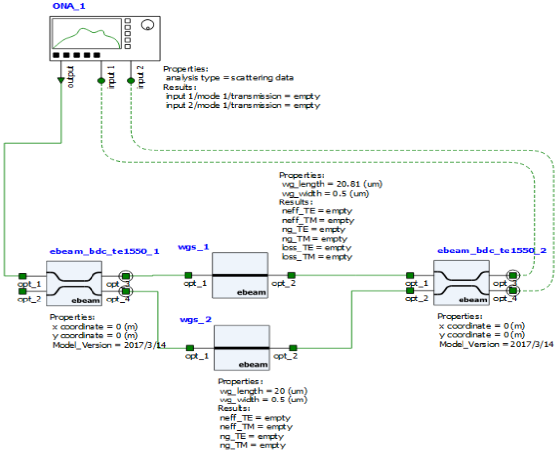
Figure 11 - Mach-Zehnder interferometer Simulation Circuit
