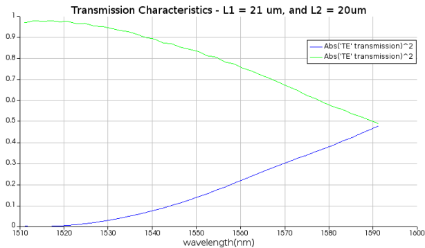
Figure 14 - Transmission characteristics L = 21 um
