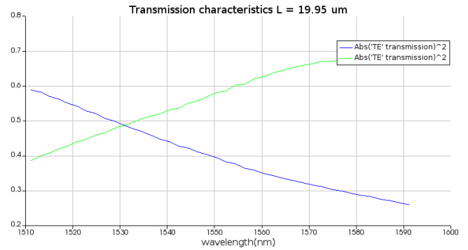
Figure 16 - Transmission characteristics L = 19.95 um
