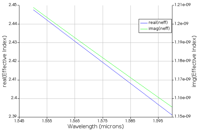
Figure 4 - Wave guide n_{\text{eff}} index.
