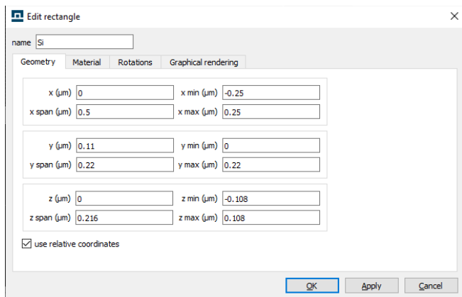
Figure 1 - Wave Guide Geometry
