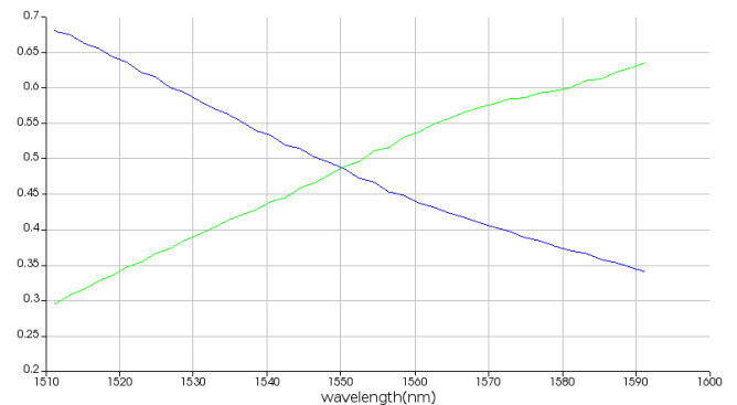
Figure 17 - Transmission characteristics L1 = 19.969 um
