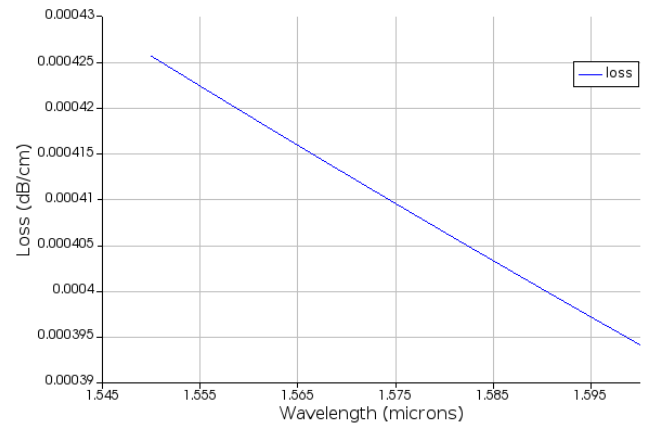
Figure 7 - Waveguide loss vs. Wavelength
