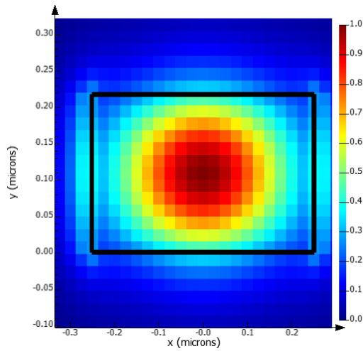
Figure 3 - Fundamental model E Intensity
