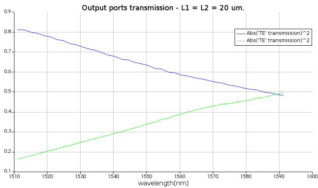
Figure 12 - Transmission characteristics - L1 = L2 = 20 um
