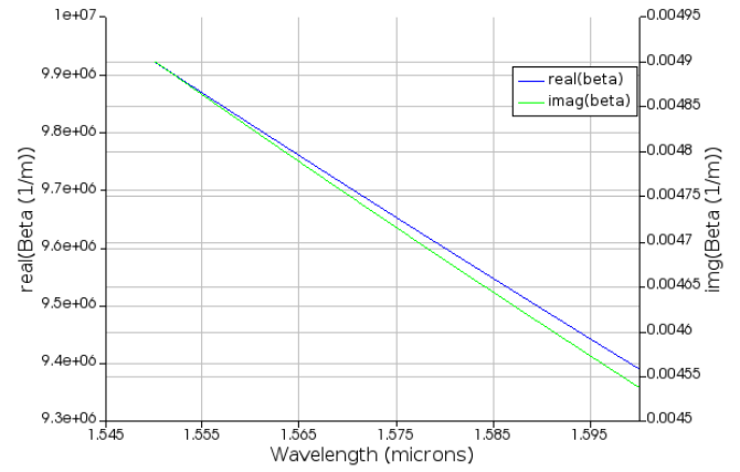
Figure 6 - Wave guide Propagation Index vs. Wavelength
